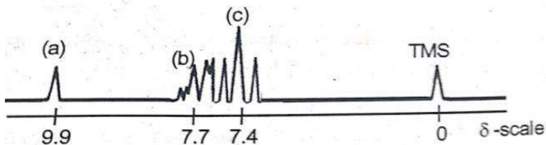
NMR spectrum of Benzaldehyde
