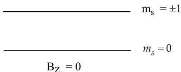
Fig. 6.17 (zero field splitting)
