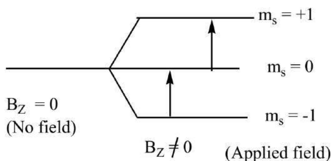
Fig. 6.16. Splitting of spin states in a magnetic field.
