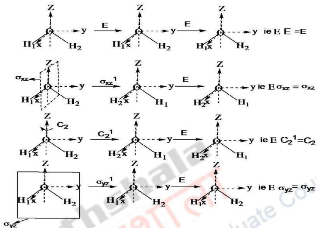
Figure 3: Combination of E with C_2 , \sigma_{xz} , \sigma_{yz}
