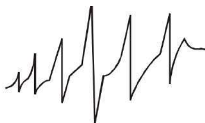
Fig.6.13. ESR spectrum of benzene anion.
