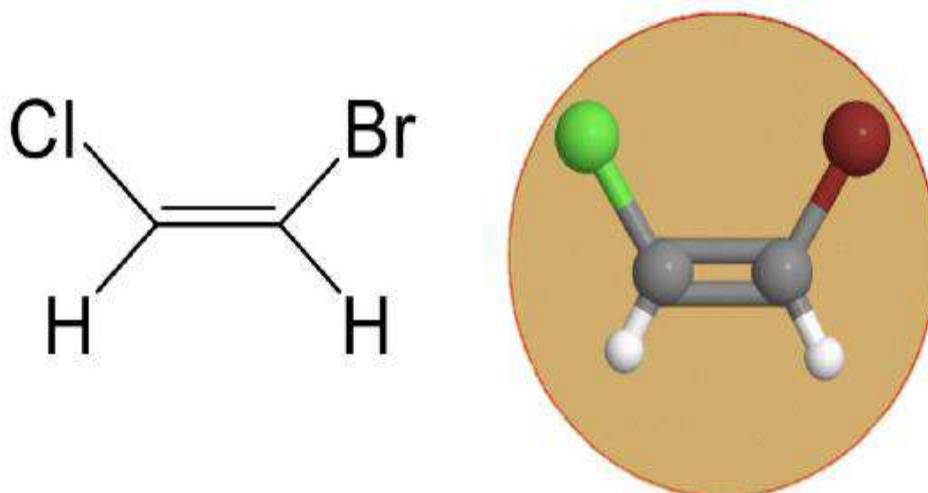
Figure 4.2.24.2.2 C_s point group of 1,2-bromochloroethene (Attribution: symotter.org/gallery)
