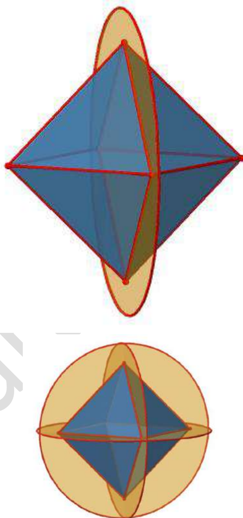
Figure 4.2.134.2.13: The horizontal mirror planes in the octahedral point group O_h (Attribution: symotter.org/gallery)
