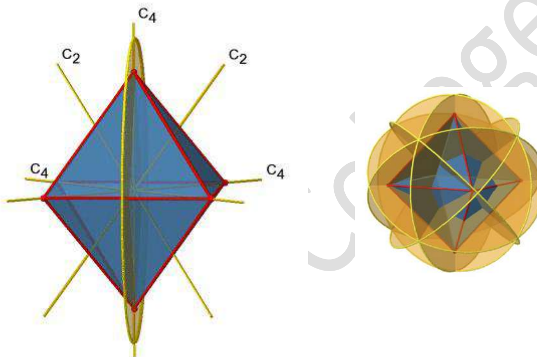
Figure 4.2.144.2.14: The vertical mirror planes in the octahedral point group O_h (Attribution: symotter.org/gallery )
