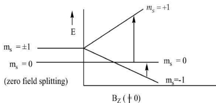
Fig. 6.18. Zero field splitting and unsymmetrical splitting of spin states giving rise to two ESR signals.
