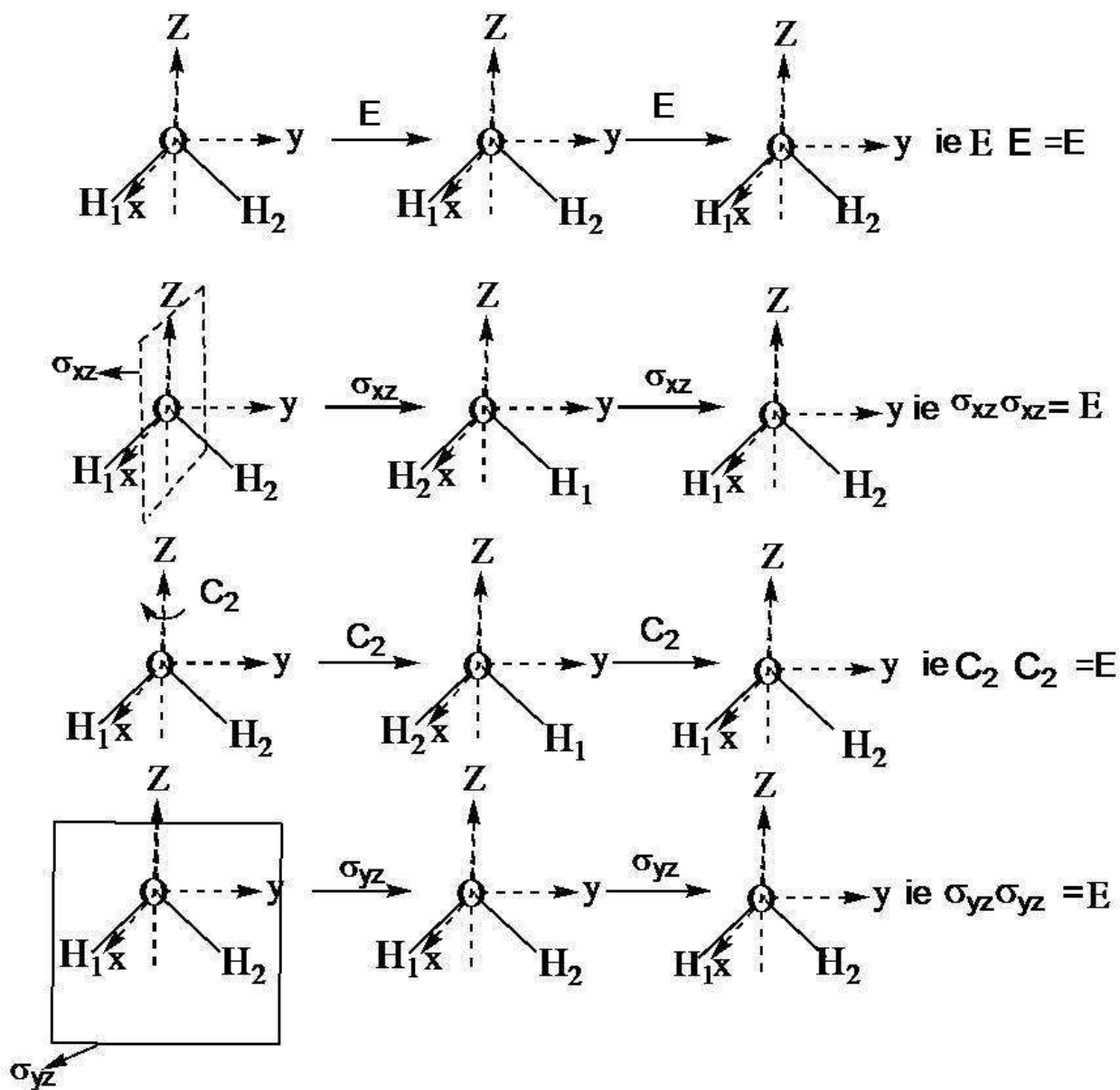
Figure 4: Combination of C 2 with C 2 , σ xz with σ xz , σ yz with σ yz
