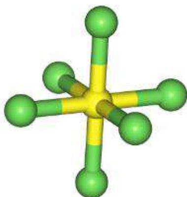
\text{SF}_6
