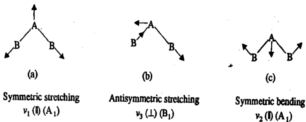
Fig.5.2: Normal modes of vibrations of a triatomic angular molecule, AB_2 (e.g., H_2O ). (a) symmetric stretching ( \nu_1 ) (b) antisymmetric stretching ( \nu_3 ) (c) symmetric bending ( \nu_2 ). \nu_1 and \nu_2 are parallel vibrations whereas \nu_3 is a perpendicular vibration.
