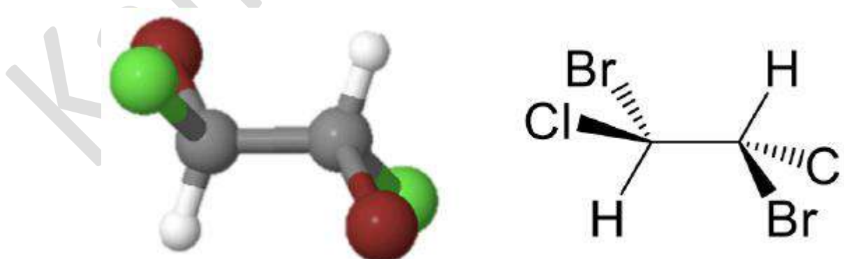
Figure 4.2.34.2.3 The C_i point group: 1,2-dibromo-1,2-dichloroethane (Attribution: symotter.org/gallery)
