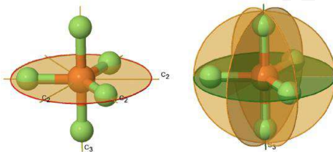
Figure 4.2.324.2.32: The \text{PF}_5 molecule belonging to the point group D_{3h} and its symmetry elements. (Attribution: symotter.org/gallery)
