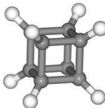
cubane
