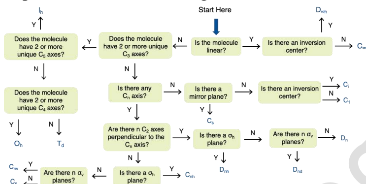
Figure 4.2.384.2.38: Flow chart for the determination of point groups. (CC BY-NC-SA; Catherine McCusker)
