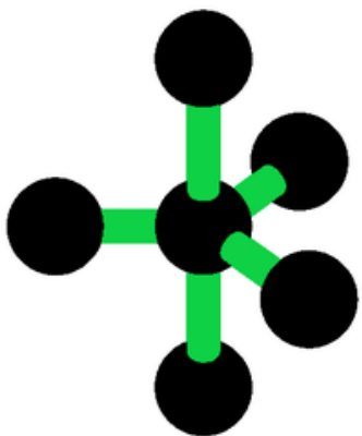
Trigonal Bipyramidal Shape
