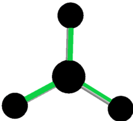
Trigonal Planar Shape
